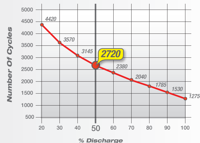
Cycle Life vs. Depth of Discharge
